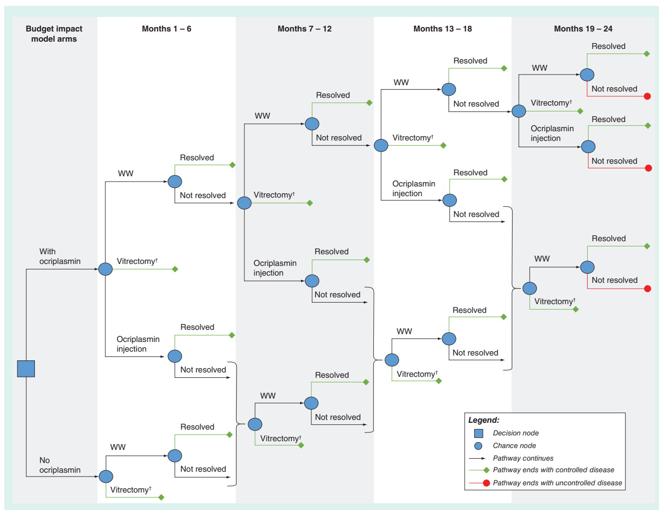
Figure 1. Analytical framework.
